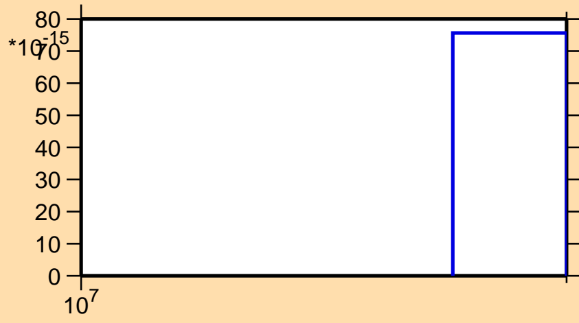
\sigma vs. E for ^{72}\text{Br}(n,nt)
