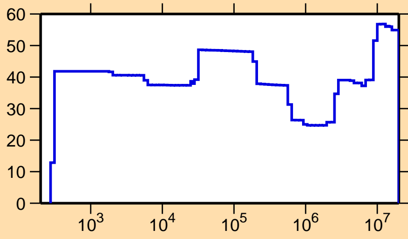
\Delta\sigma/\sigma vs. E for ^{72}\text{Br}(n,p)
