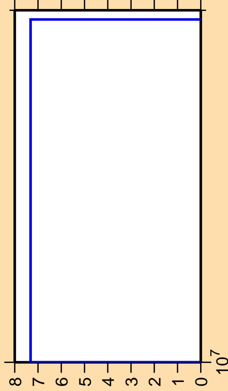
\Delta\sigma/\sigma vs. E for ^{72}\text{Br}(n,2n\alpha)
