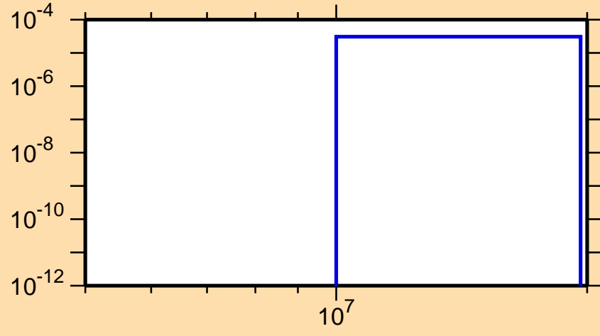
\sigma vs. E for ^{72}\text{Br} (mt 45)
