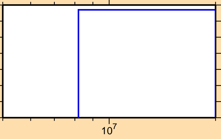
\sigma vs. E for ^{72}\text{Br}(n,\text{nd})
