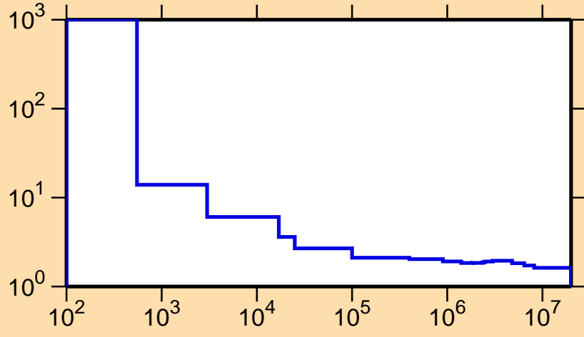
\sigma vs. E for ^{72}\text{Br}(n,\text{nonel.})
