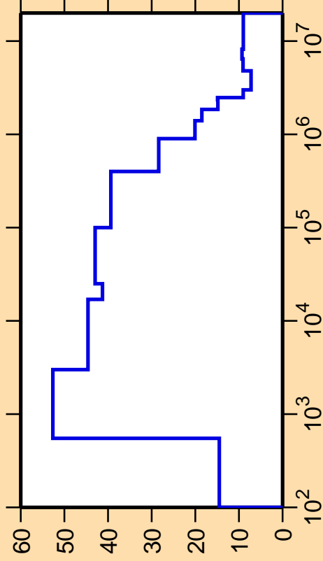
\Delta\sigma/\sigma vs. E for ^{72}\text{Br}(n,\text{nonel.})
