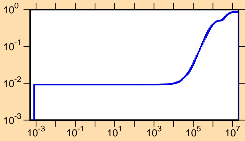
\mu vs. E for ^{73}\text{Br}(\text{mt251})
