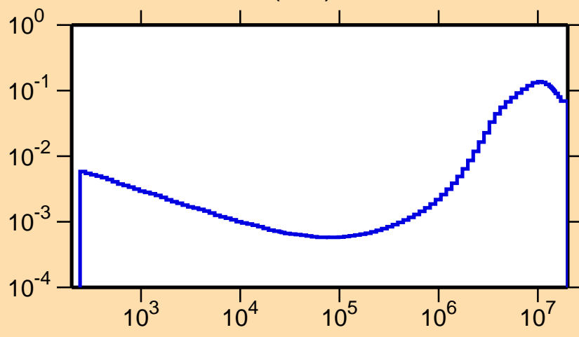
\sigma vs. E for ^{73}\text{Br}(n,\alpha)
