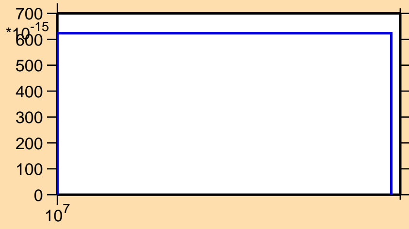
\sigma vs. E for ^{73}\text{Br}(n,nt)
