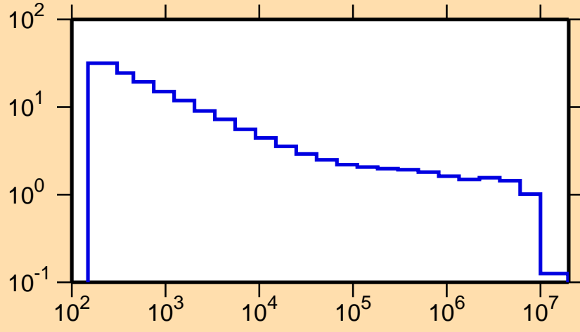
\sigma vs. E for ^{73}\text{Br}(n,p)
