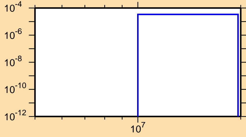
\sigma vs. E for ^{73}\text{Br} (mt 45)
