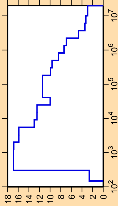
\Delta\sigma/\sigma vs. E for ^{73}\text{Br}(n,\text{nonel.})
