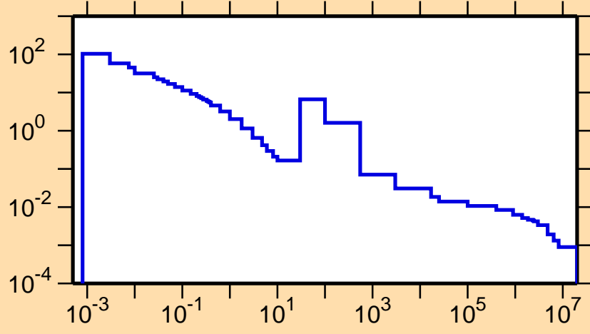
\sigma vs. E for ^{73}\text{Br}(n,\gamma)
