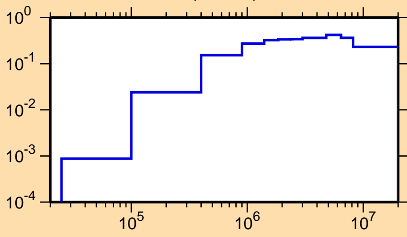
\sigma vs. E for ^{73}\text{Br}(n,\text{inel.})
