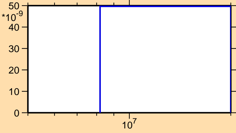
\sigma vs. E for ^{73}\text{Br}(n,\text{nd})
