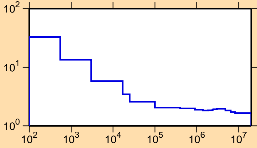
\sigma vs. E for ^{73}\text{Br}(n,\text{nonel.})
