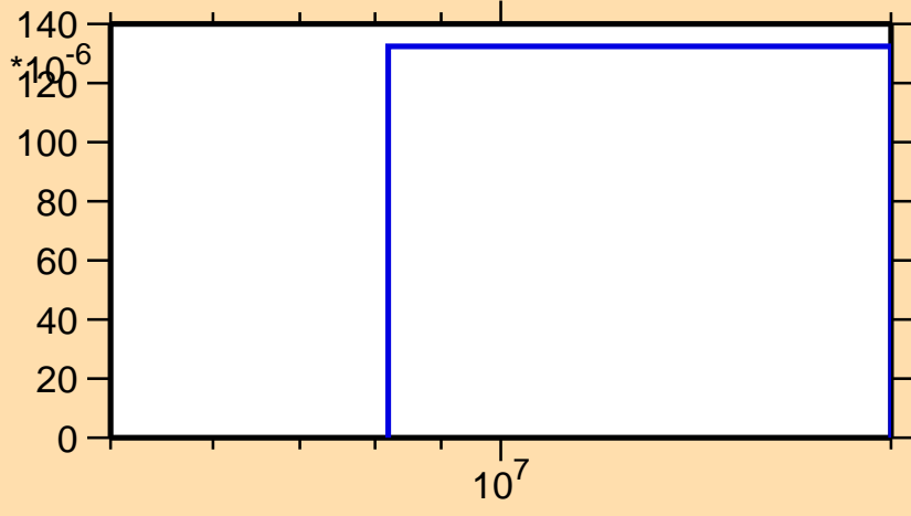
\sigma vs. E for ^{73}\text{Br}(n,t)
