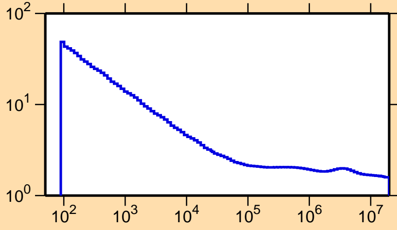
\sigma vs. E for ^{74}\text{Br}(n,\text{nonel.})
