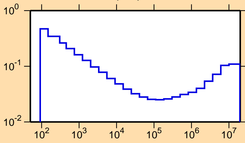
\sigma vs. E for ^{74}\text{Br}(n,\alpha)
