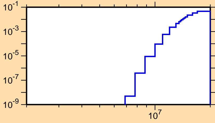
\sigma vs. E for ^{74}\text{Br}(n,n\alpha)
