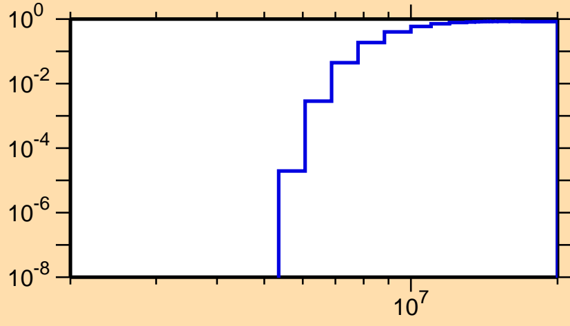
\sigma vs. E for ^{74}\text{Br}(n,np)
