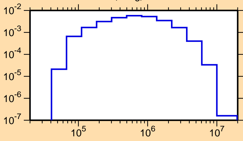
\sigma vs. E for ^{74}\text{Br}(n,n_3)
