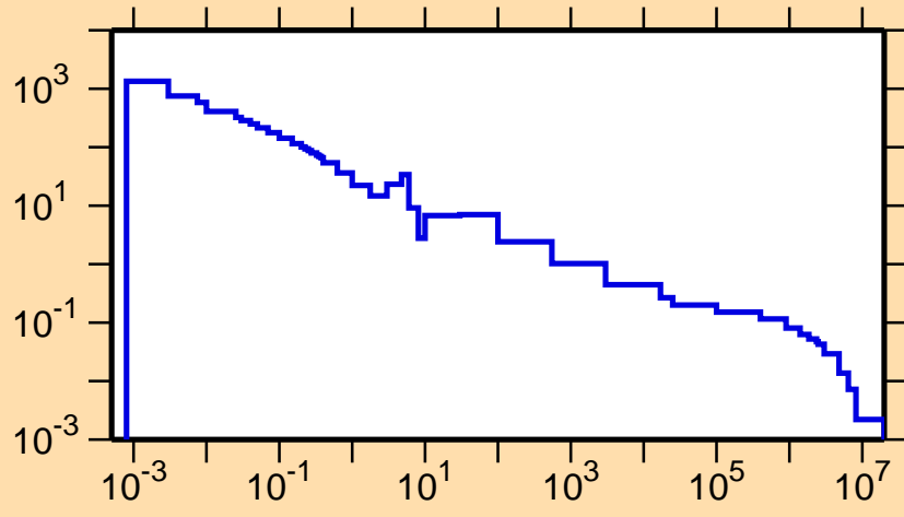
\sigma vs. E for ^{74}\text{Br}(n,\gamma)
