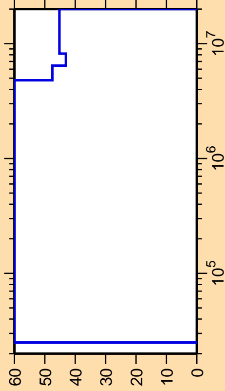
\Delta\sigma/\sigma vs. E for ^{74}\text{Br}(n,n_3)
