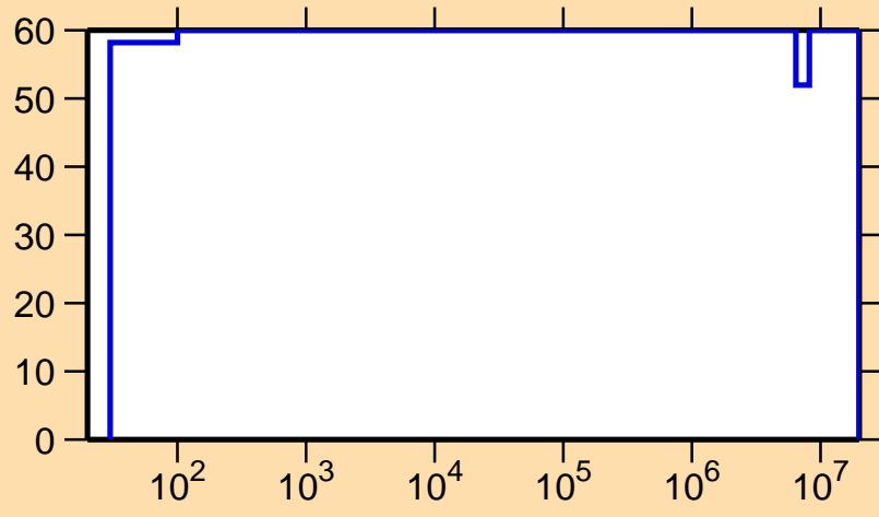
\Delta\sigma/\sigma vs. E for ^{74}\text{Br}(n,\gamma)
