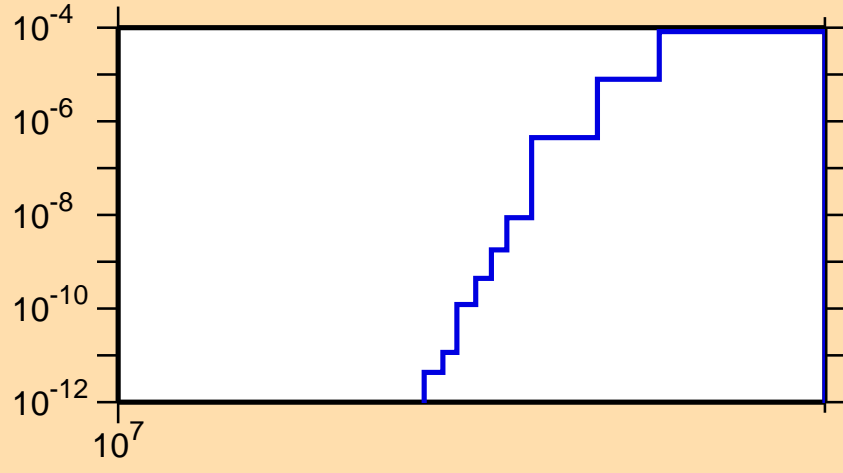
\sigma vs. E for ^{75}\text{Br}(n,\text{pd})
