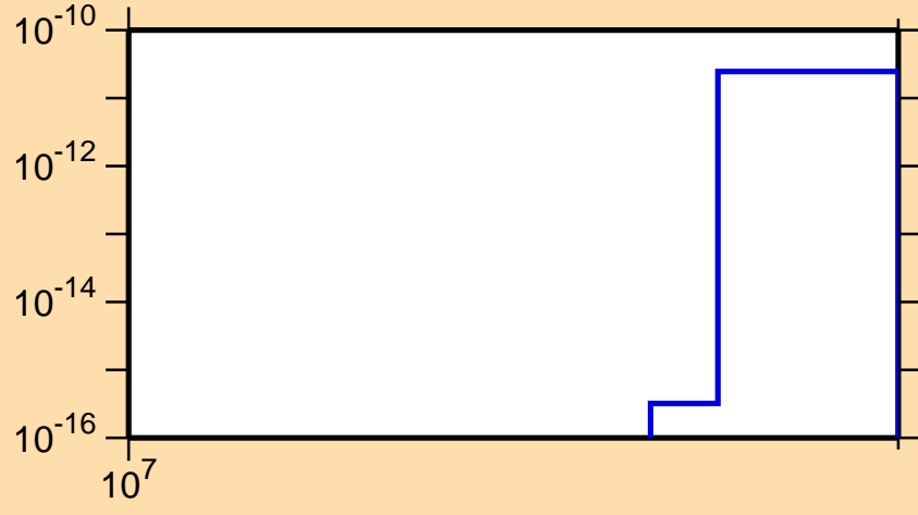
\sigma vs. E for ^{75}\text{Br}(n,\text{pt})
