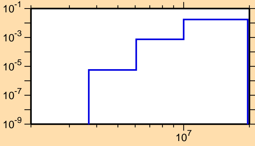
\sigma vs. E for ^{75}\text{Br}(n,d)
