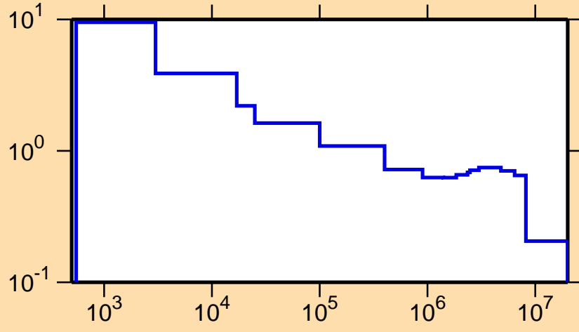
\sigma vs. E for ^{75}\text{Br}(n,p)
