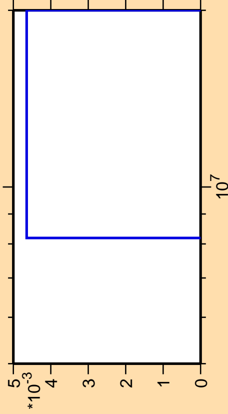
\Delta\sigma/\sigma vs. E for ^{75}\text{Br} (mt 34)
