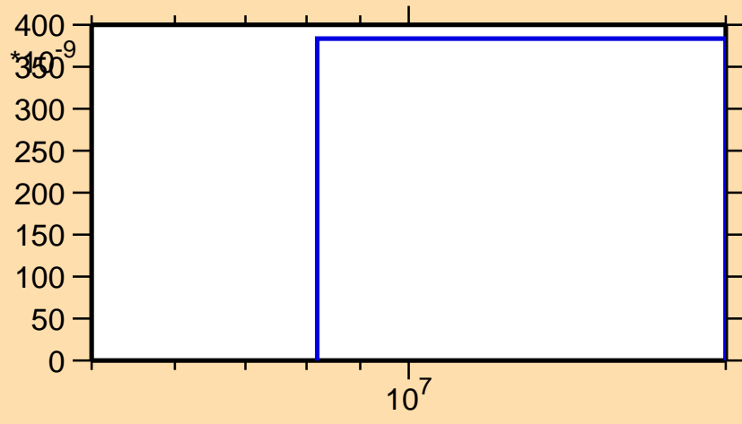
\sigma vs. E for ^{75}\text{Br} (mt 45)
