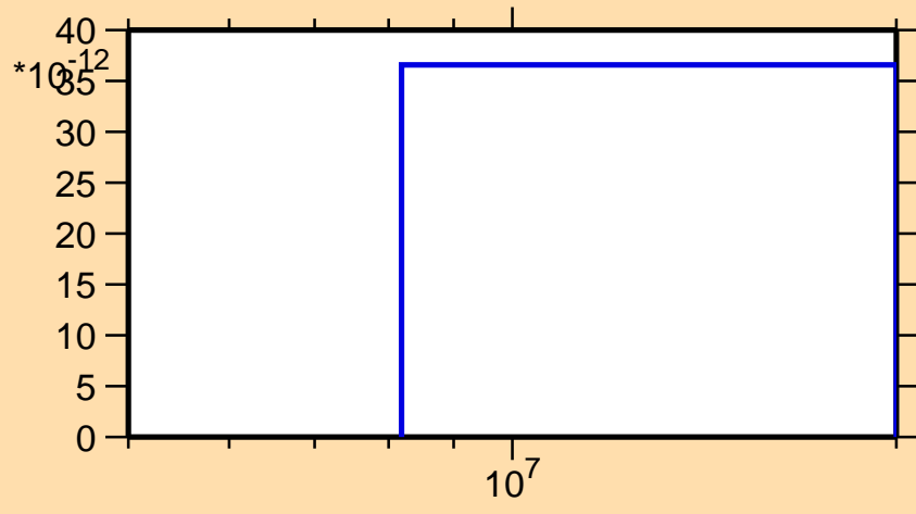
\sigma vs. E for ^{75}\text{Br}(n,nt)
