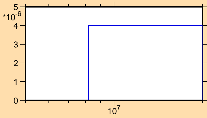
\sigma vs. E for ^{75}\text{Br}(n,\text{He}3)
