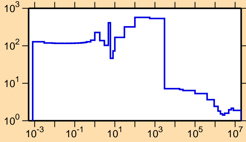
\sigma vs. E for ^{75}\text{Br}(n,\text{el.})
