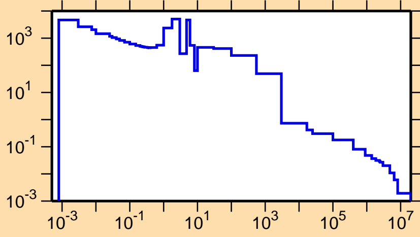
\sigma vs. E for ^{75}\text{Br}(n,\gamma)
