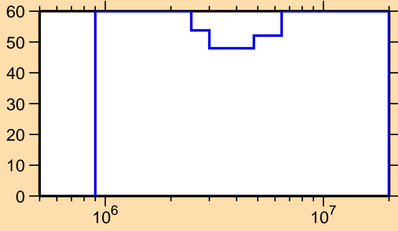
\Delta\sigma/\sigma vs. E for ^{75}\text{Br}(n,n\text{cont.})
