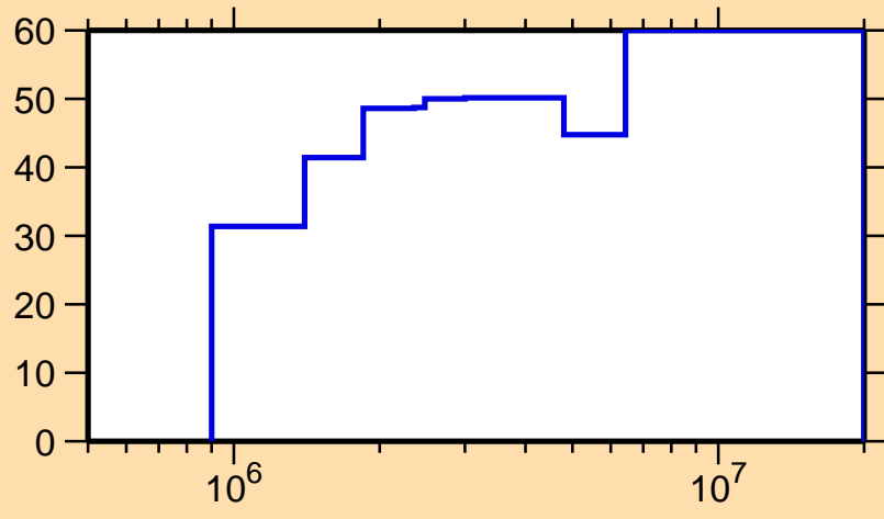
\Delta\sigma/\sigma vs. E for ^{75}\text{Br}(n,n_1)
