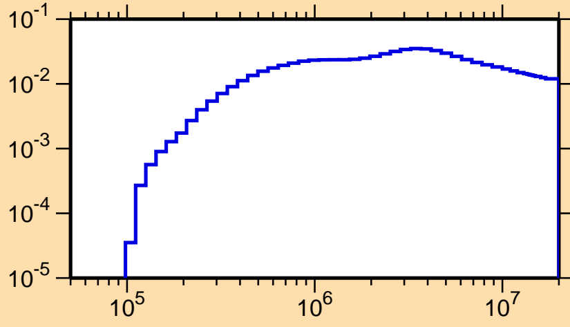
\sigma vs. E for ^{76}\text{Br}(n,n_2)
