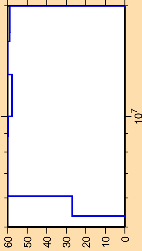
\Delta\sigma/\sigma vs. E for ^{76}\text{Br}(n,np)
