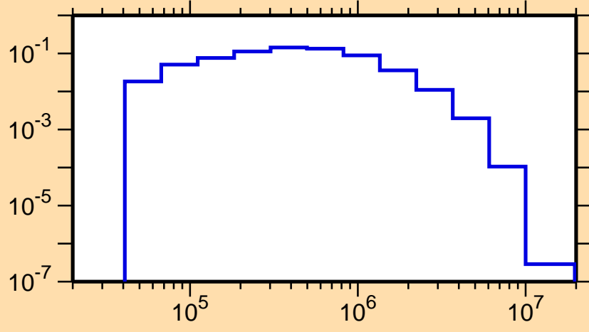
\sigma vs. E for ^{76}\text{Br}(n,n_1)
