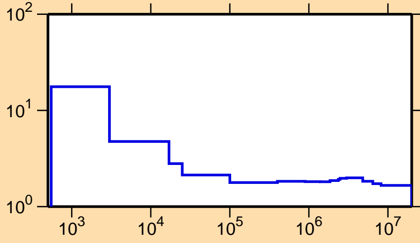
\sigma vs. E for ^{76}\text{Br}(n,\text{nonel.})
