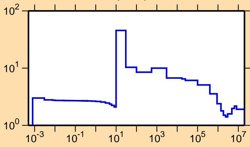
\sigma vs. E for ^{76}\text{Br}(n,\text{el.})
