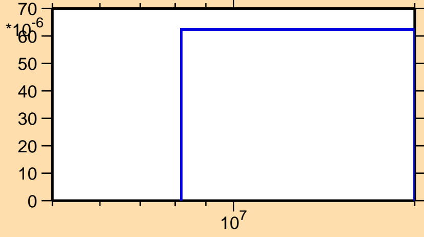
\sigma vs. E for ^{77}\text{Br}(n,t)
