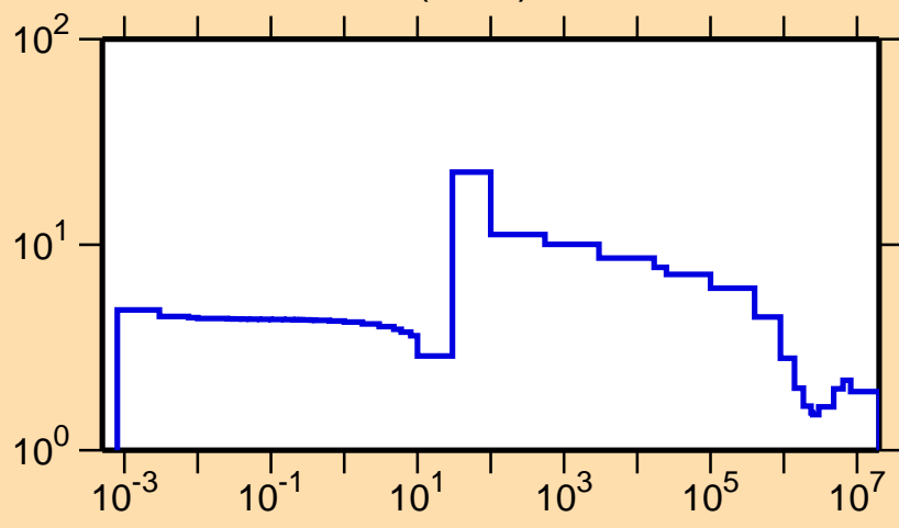
\sigma vs. E for ^{77}\text{Br}(n,\text{el.})
