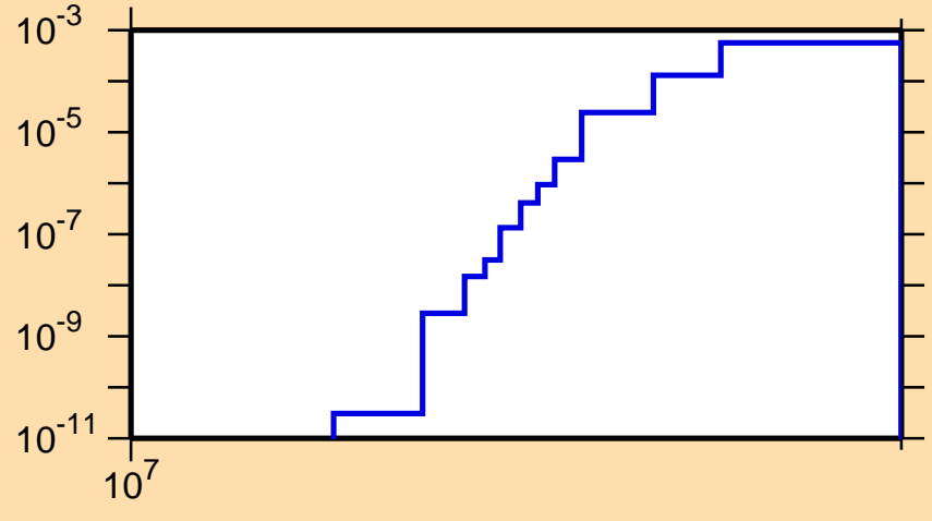
\sigma vs. E for ^{78}\text{Br}(n,nd)
