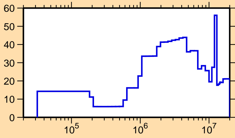
\Delta\sigma/\sigma vs. E for ^{78}\text{Br}(n,n_1)
