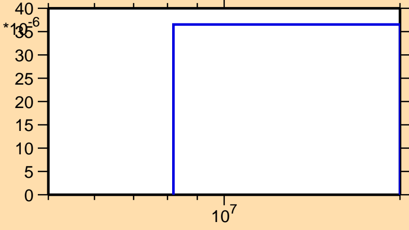
\sigma vs. E for ^{79}\text{Br}(n,t)
