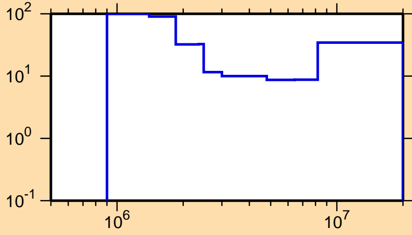
\Delta\sigma/\sigma vs. E for ^{79}\text{Br}(n,n\text{cont.})
