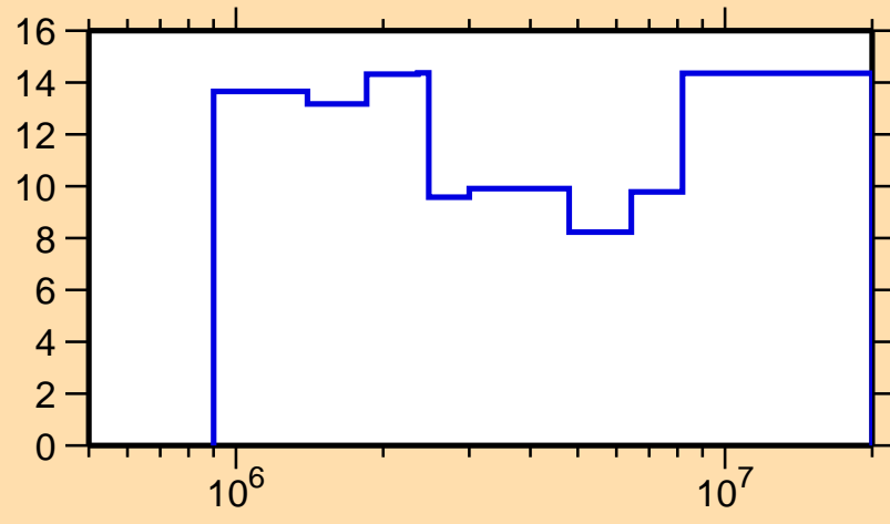
\Delta\sigma/\sigma vs. E for ^{79}\text{Br}(n,el.)
