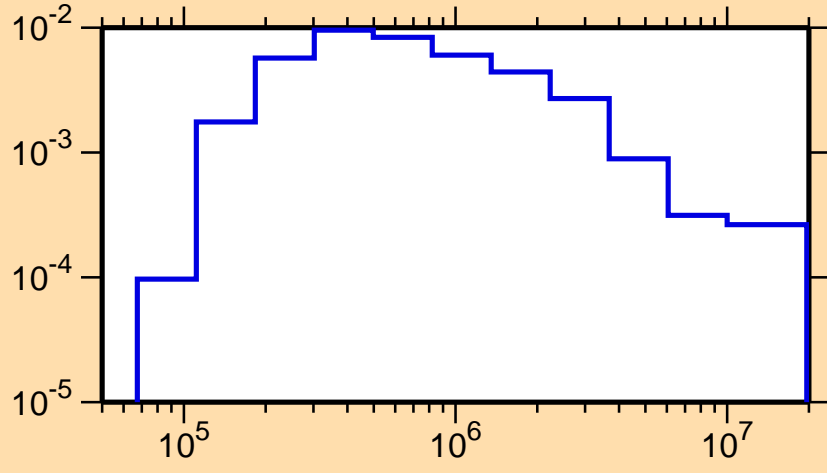
\sigma vs. E for ^{80}\text{Br}(n,n_2)
