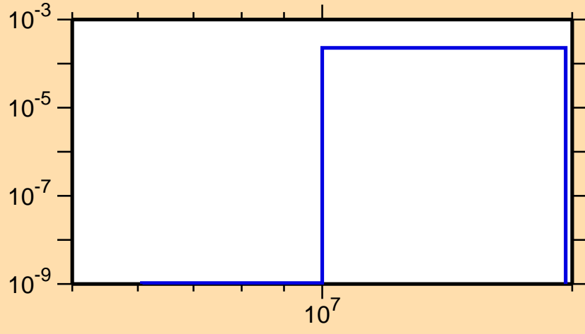
\sigma vs. E for ^{80}\text{Br}(n,t)
