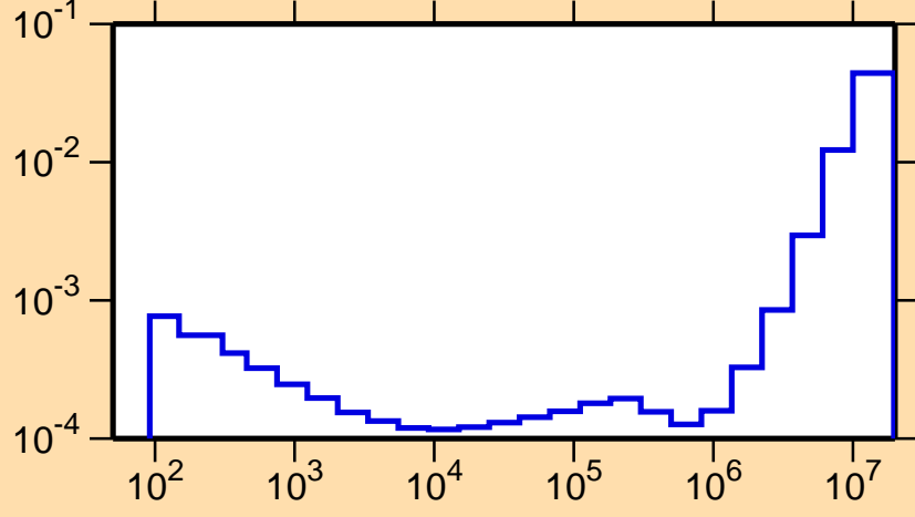
\sigma vs. E for ^{80}\text{Br}(n,p)
