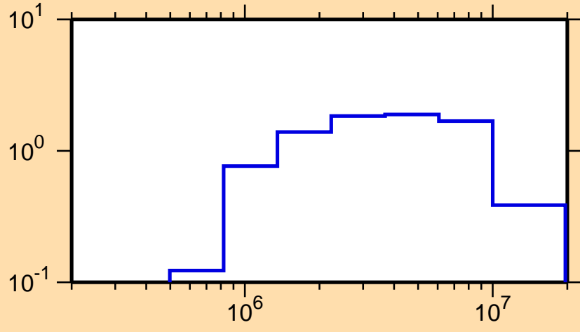
\sigma vs. E for ^{80}\text{Br}(n,n\text{cont.})
