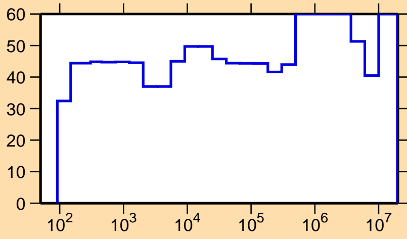
\Delta\sigma/\sigma vs. E for ^{80}\text{Br}(n,\gamma)
