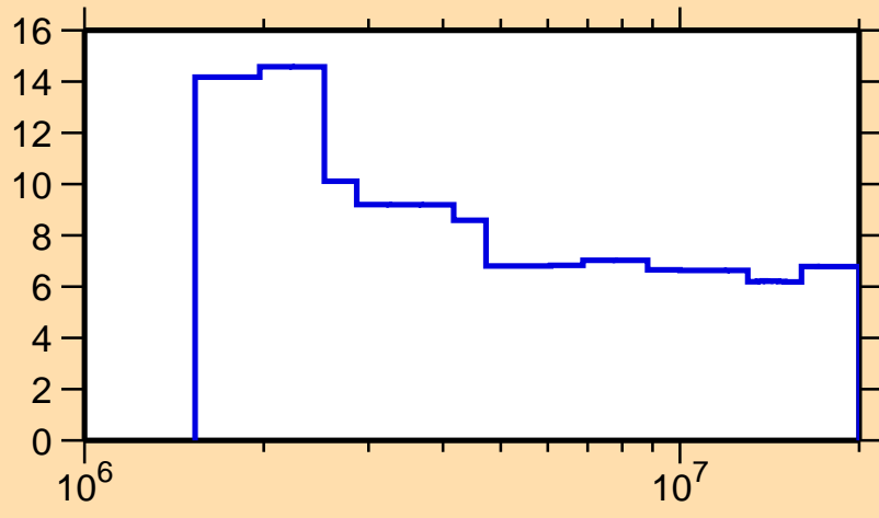
\Delta\sigma/\sigma vs. E for ^{81}\text{Br}(n,n\text{onel.})
