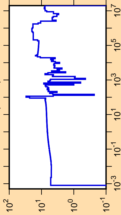
\Delta\sigma/\sigma vs. E for ^{81}\text{Br}(n,\text{tot.})
