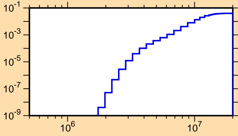
\sigma vs. E for ^{81}\text{Br}(n,p)
