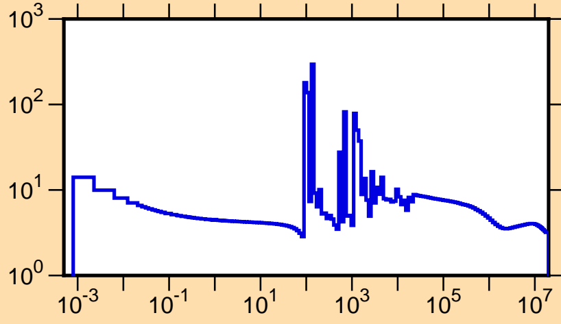
\sigma vs. E for ^{81}\text{Br}(n,\text{tot.})
