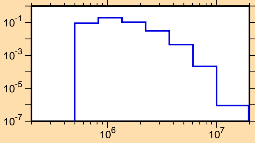
\sigma vs. E for ^{81}\text{Br}(n,n_4)
