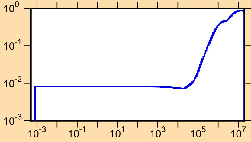
\mu vs. E for ^{82}\text{Br}(\text{mt251})
