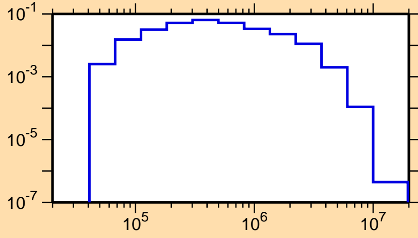
\sigma vs. E for ^{82}\text{Br}(n,n_1)
