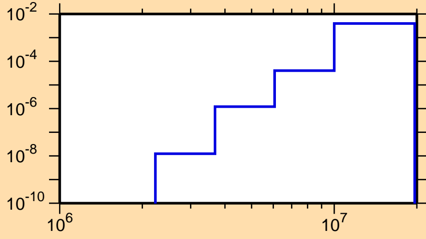
\sigma vs. E for ^{82}\text{Br}(n,\alpha)
