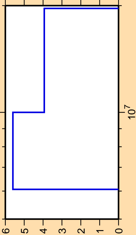
\Delta\sigma/\sigma vs. E for ^{82}\text{Br}(n,2n)
