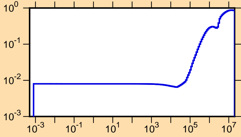
\mu vs. E for ^{84}\text{Br}(\text{mt251})
