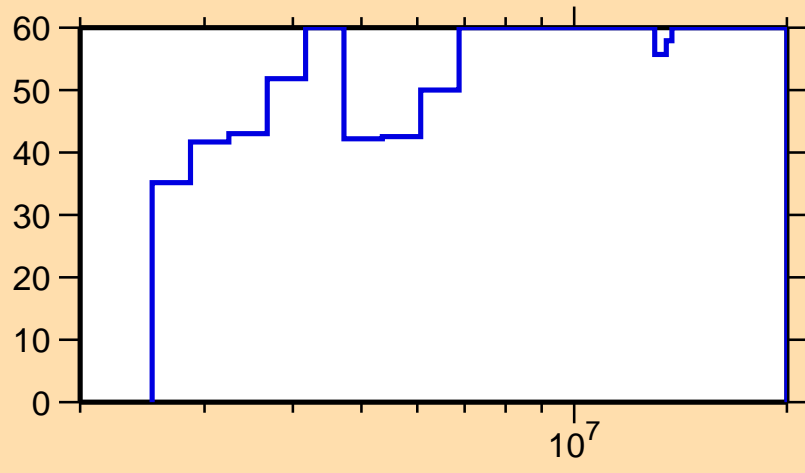
\Delta\sigma/\sigma vs. E for ^{84}\text{Br}(n,n_1)
