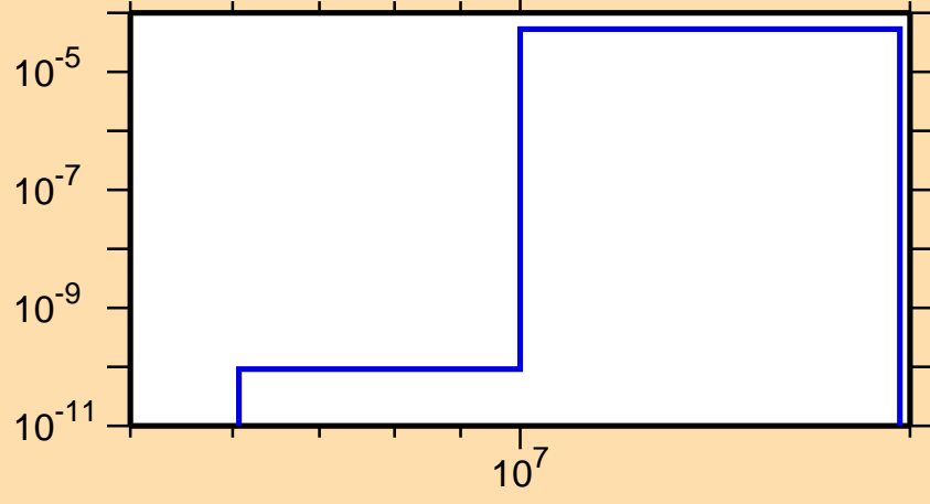
\sigma vs. E for ^{84}\text{Br}(n,t)
