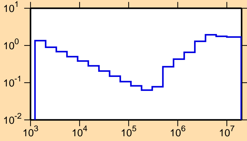
\sigma vs. E for ^{84}\text{Br}(n,\text{nonel.})
