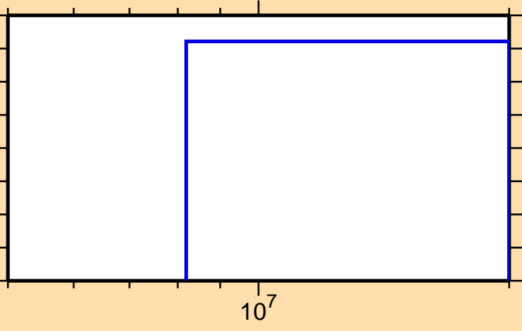
\sigma vs. E for ^{84}\text{Br}(n,\text{He}3)
