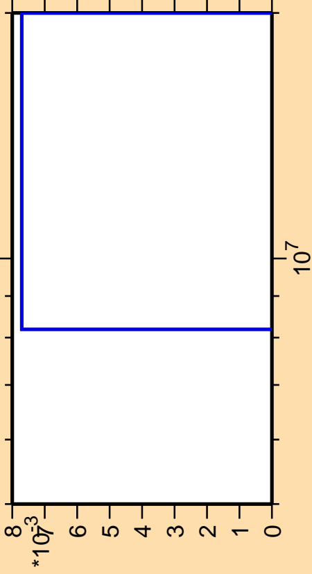
\Delta\sigma/\sigma vs. E for ^{84}\text{Br}(n,p\alpha)
