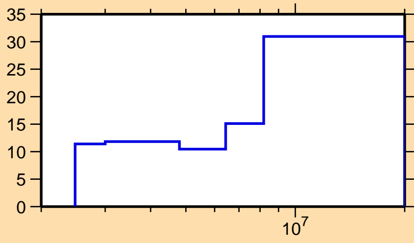
\Delta\sigma/\sigma vs. E for ^{84}\text{Br}(n,ncont.)
