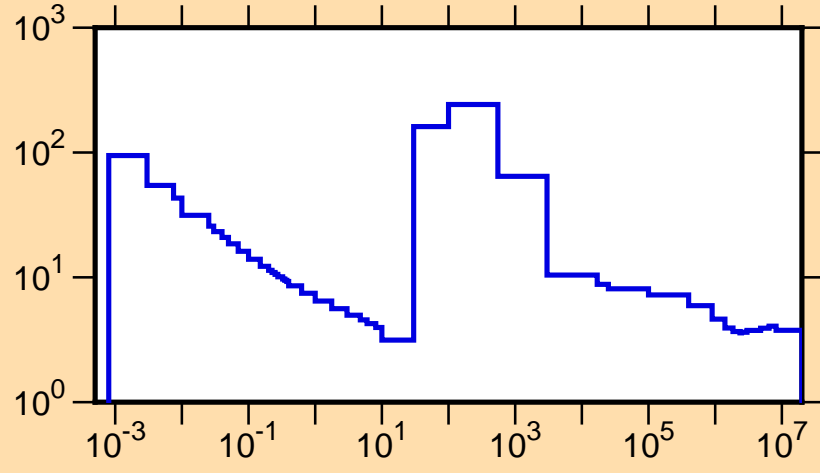
\sigma vs. E for ^{84}\text{Br}(n,\text{tot.})
