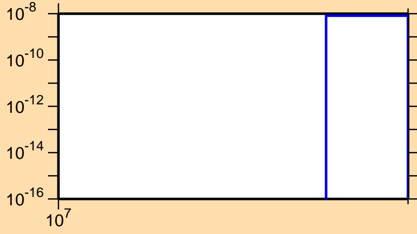
\sigma vs. E for ^{85}\text{Br}(n,nt)
