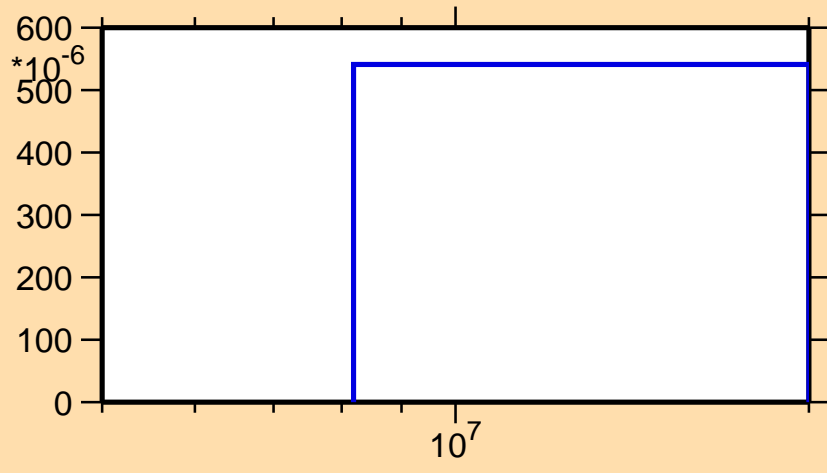
\sigma vs. E for ^{85}\text{Br}(n,d)
