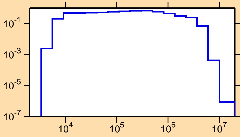
\sigma vs. E for ^{86}\text{Br}(n,n_1)
