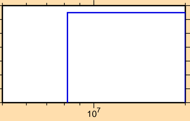
\sigma vs. E for ^{86}\text{Br}(n,3n)
