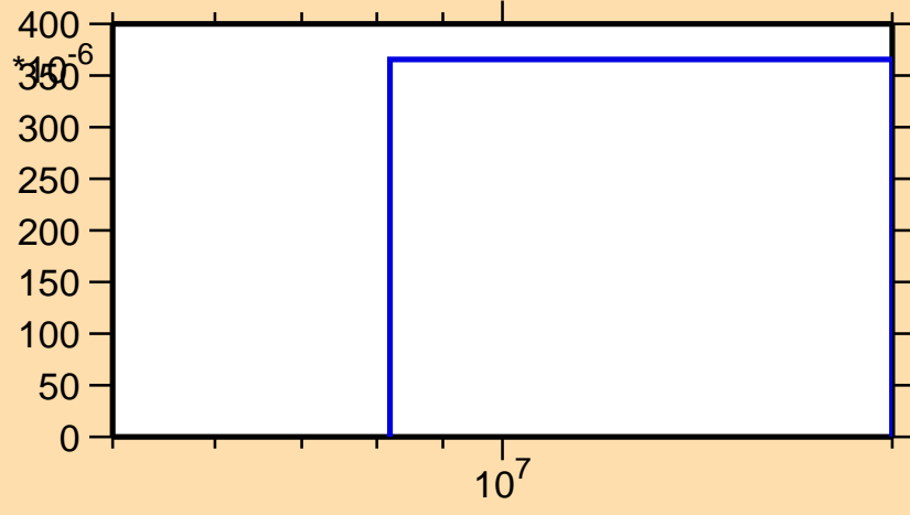
\sigma vs. E for ^{86}\text{Br}(n,d)
