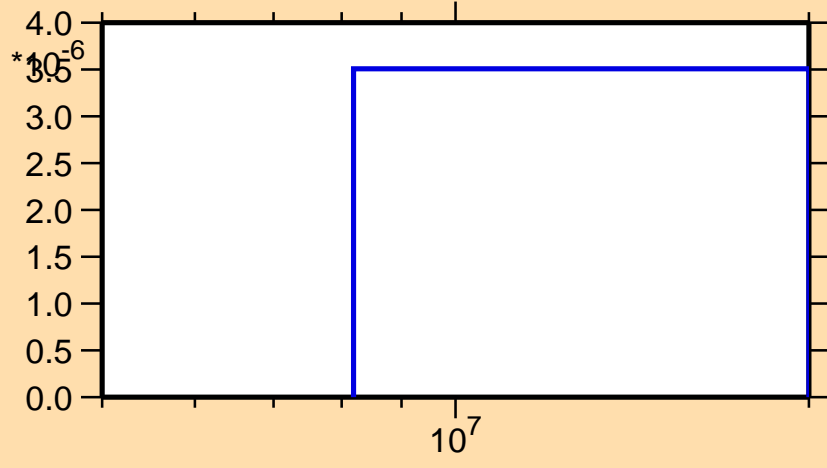
\sigma vs. E for ^{86}\text{Br}(n,\alpha)
