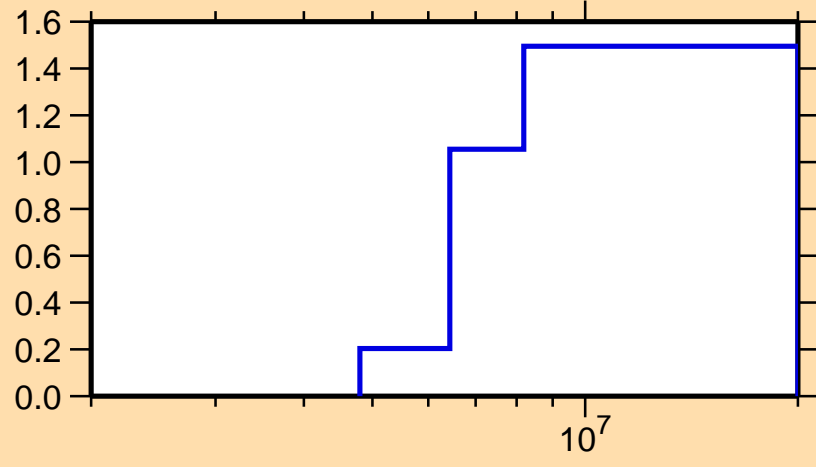
\sigma vs. E for ^{86}\text{Br}(n,2n)
