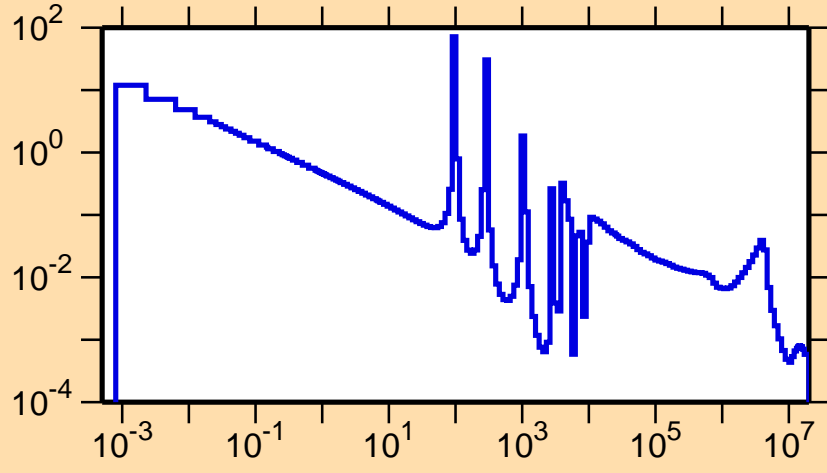
\sigma vs. E for ^{87}\text{Br}(n,\gamma)
