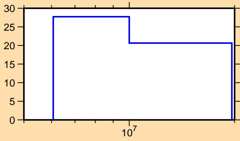
\Delta\sigma/\sigma vs. E for ^{87}\text{Br}(n,2n)
