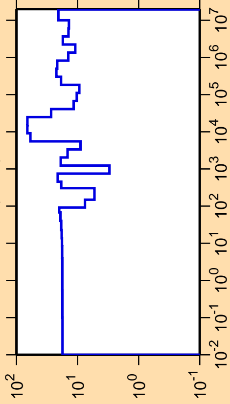
\Delta\sigma/\sigma vs. E for ^{87}\text{Br}(n,\text{el.})
