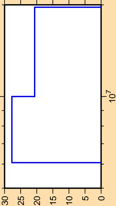
\Delta\sigma/\sigma vs. E for ^{87}\text{Br}(n,2n)
