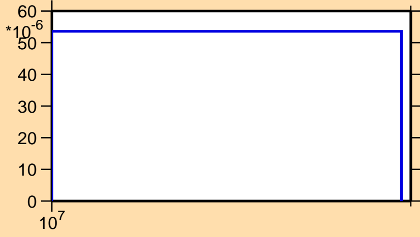
\sigma vs. E for ^{87}\text{Br}(n,np)
