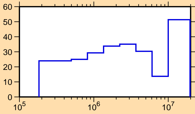
\Delta\sigma/\sigma vs. E for ^{87}\text{Br}(n,\text{inel.})
