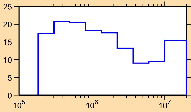
\Delta\sigma/\sigma vs. E for ^{87}\text{Br}(n,\text{tot.})
