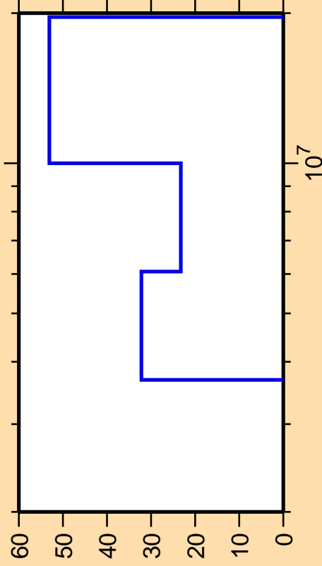
\Delta\sigma/\sigma vs. E for ^{87}\text{Br}(n,ncont.)
