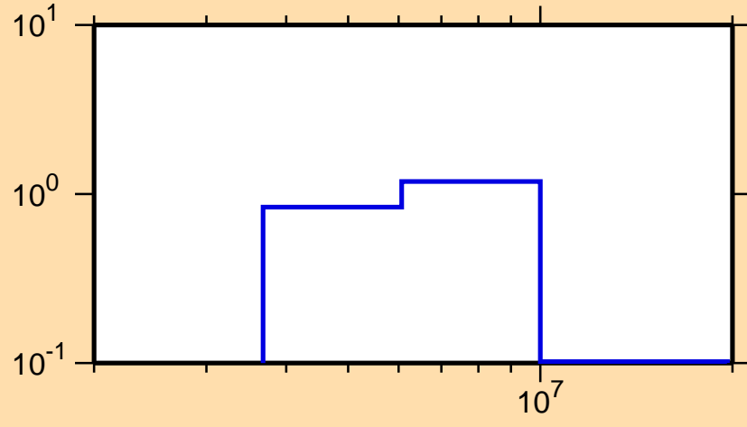
\sigma vs. E for ^{87}\text{Br}(n,n\text{cont.})
