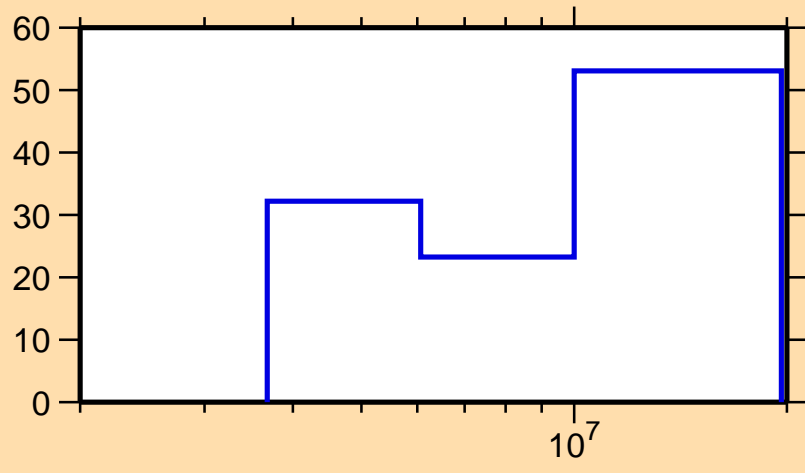
\Delta\sigma/\sigma vs. E for ^{87}\text{Br}(n,n\text{cont.})
