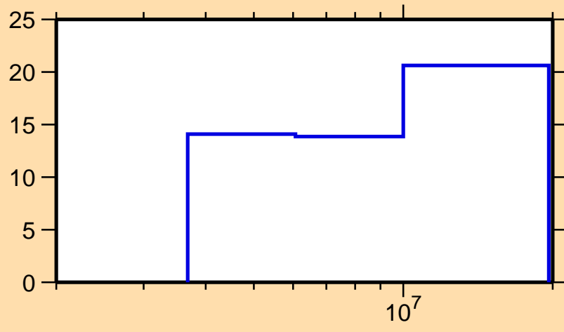
\Delta\sigma/\sigma vs. E for ^{87}\text{Br}(n,\text{el.})
