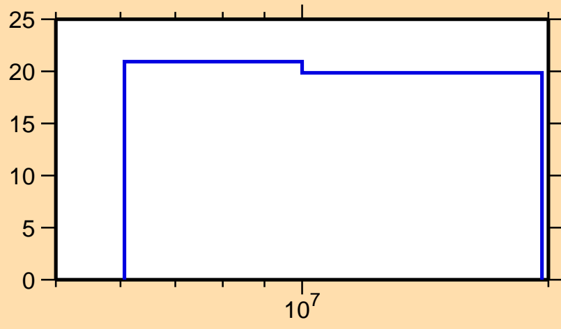
\Delta\sigma/\sigma vs. E for ^{87}\text{Br}(n,\text{nonel.})
