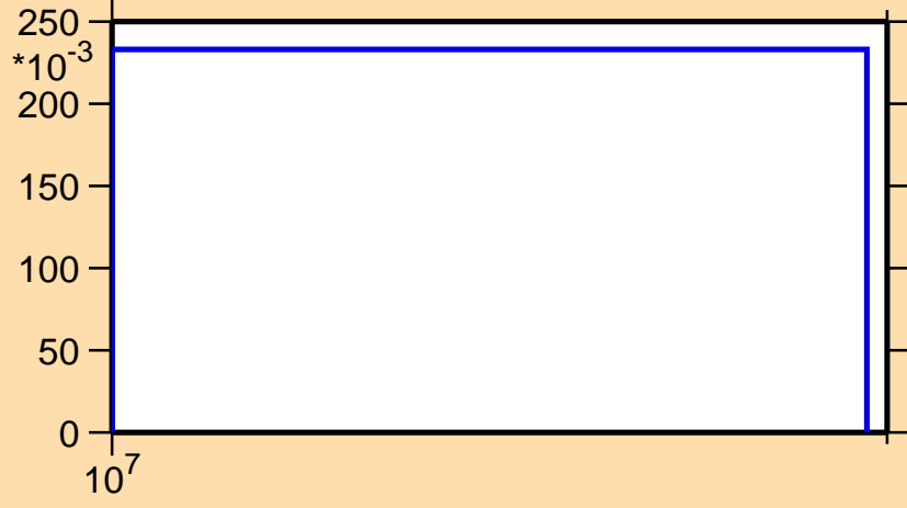
\sigma vs. E for ^{87}\text{Br}(n,3n)
