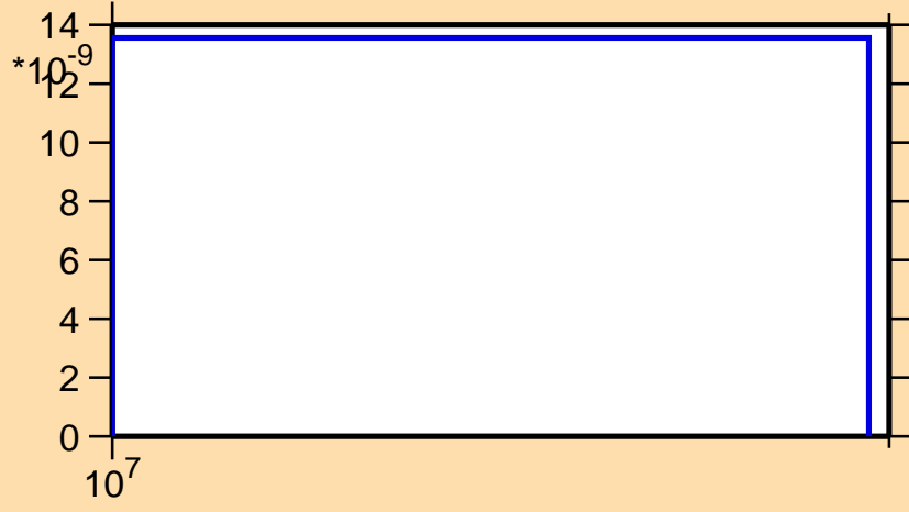
\sigma vs. E for ^{87}\text{Br}(n,\text{nd})
