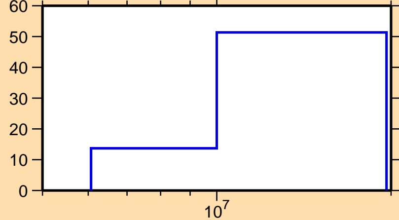
\Delta\sigma/\sigma vs. E for ^{87}\text{Br}(n,\text{inel.})
