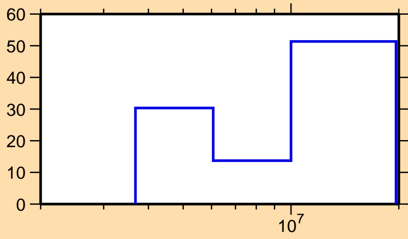
\Delta\sigma/\sigma vs. E for ^{87}\text{Br}(n,inel.)
