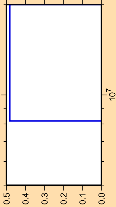
\Delta\sigma/\sigma vs. E for ^{87}\text{Br}(n,2n\alpha)
