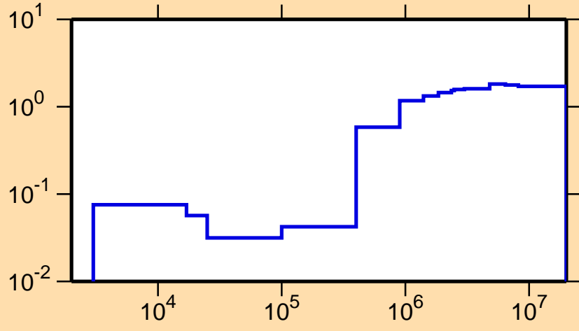
\sigma vs. E for ^{87}\text{Br}(n,\text{nonel.})
