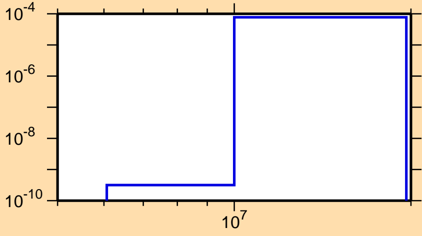
\sigma vs. E for ^{90}\text{Br}(n,t)
