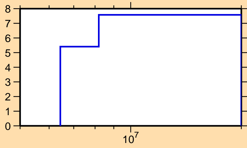
\Delta\sigma/\sigma vs. E for ^{90}\text{Br}(n,\text{tot.})
