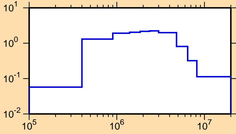
\sigma vs. E for ^{90}\text{Br}(n,\text{inel.})
