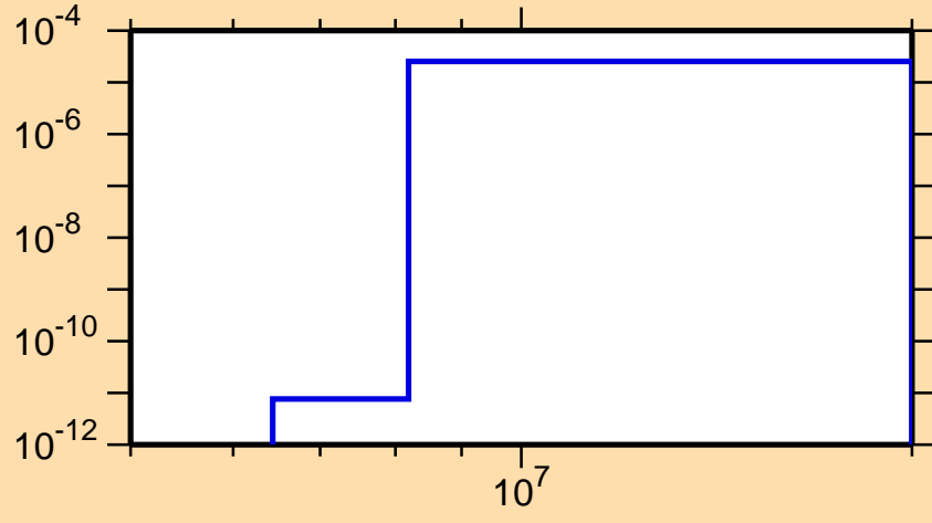
\sigma vs. E for ^{90}\text{Br}(n,\alpha)
