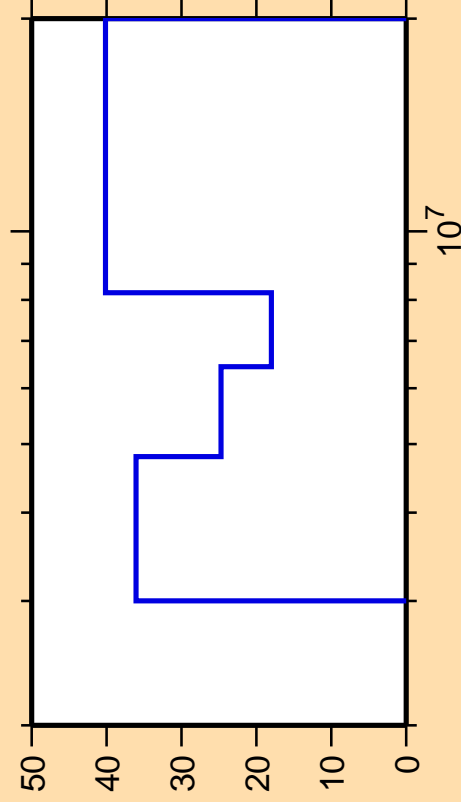
\Delta\sigma/\sigma vs. E for ^{90}\text{Br}(n,2n)
