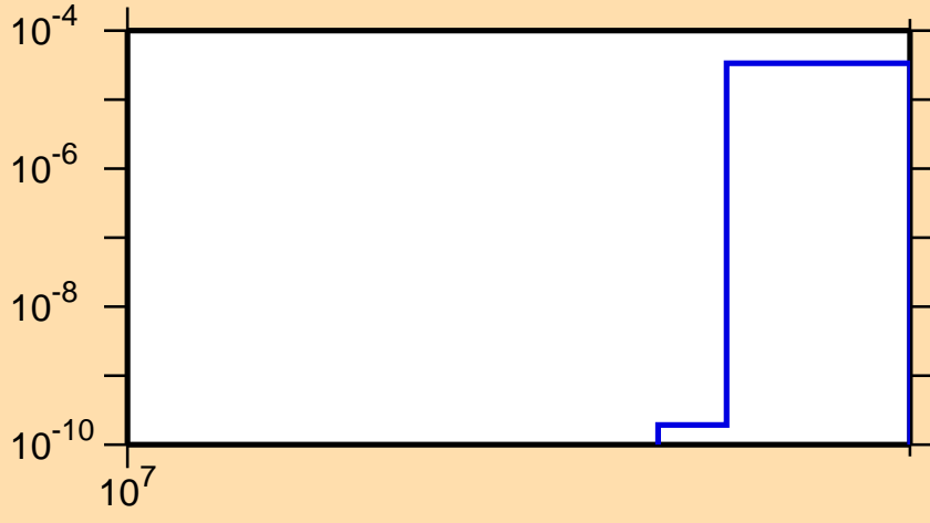
\sigma vs. E for ^{10}\text{C} (mt 34)
