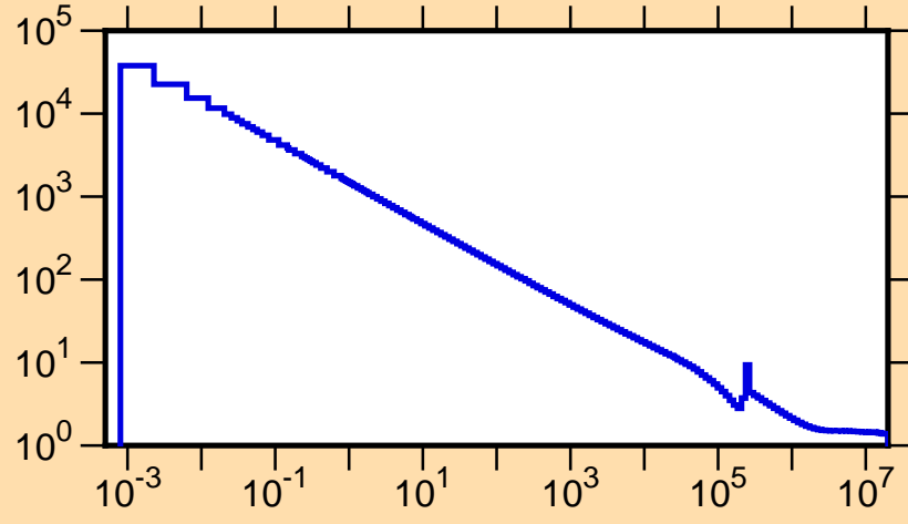
\sigma vs. E for ^{10}\text{C}(n,\text{tot.})
