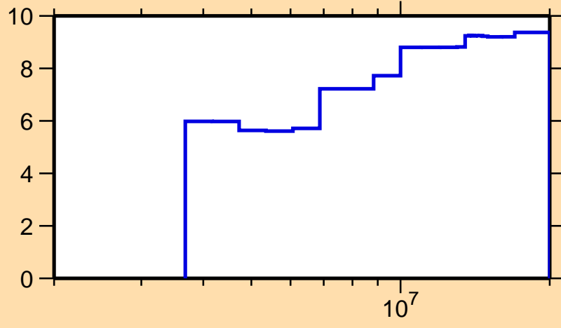
\Delta\sigma/\sigma vs. E for ^{10}\text{C}(n,\text{nonel.})
