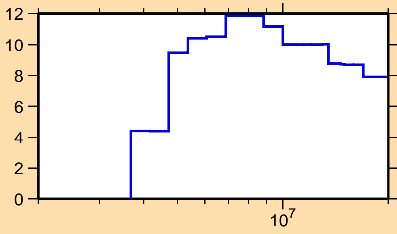
\Delta\sigma/\sigma vs. E for ^{10}\text{C}(n,\text{el.})
