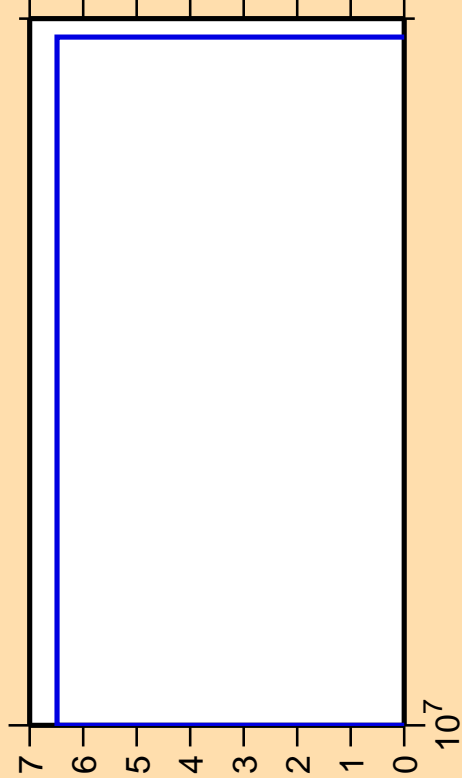
\Delta\sigma/\sigma vs. E for ^{10}\text{C}(n,t)
