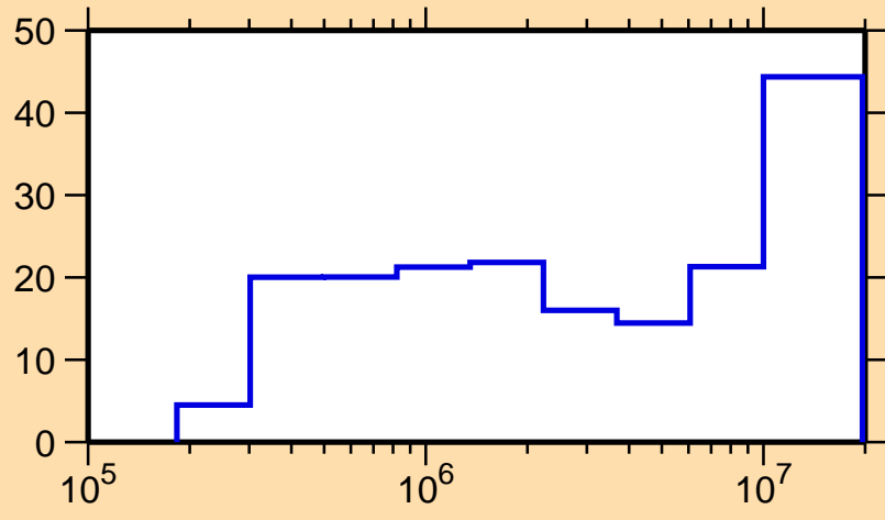
\Delta\sigma/\sigma vs. E for ^{10}\text{C}(n,p)
