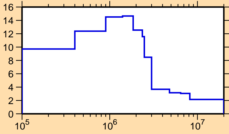
\Delta\sigma/\sigma vs. E for ^{10}\text{C}(n,\text{tot.})
