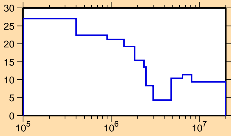
\Delta\sigma/\sigma vs. E for ^{10}\text{C}(n,el.)
