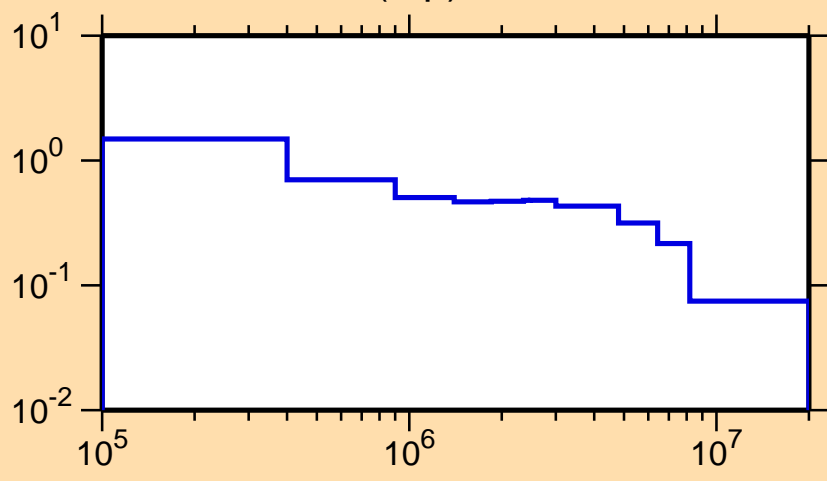
\sigma vs. E for ^{10}\text{C}(n,p)
