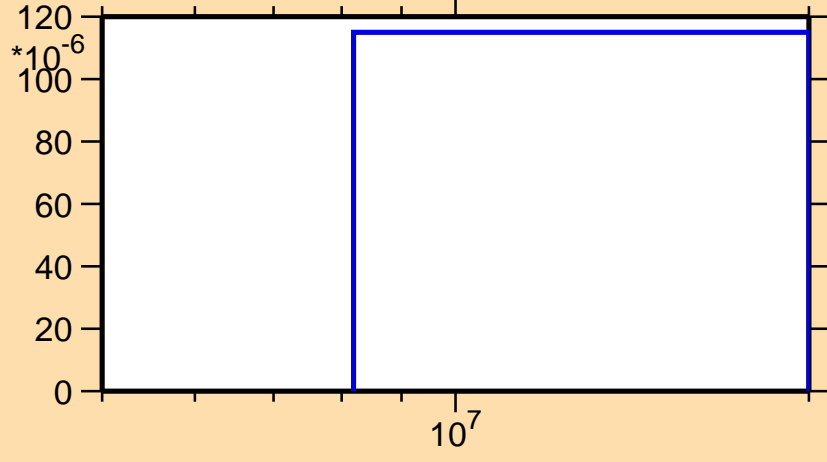
\sigma vs. E for ^{10}\text{C}(n,n\alpha)
