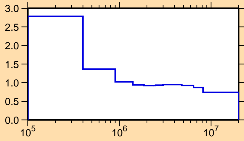
\sigma vs. E for ^{10}\text{C}(n,\text{nonel.})
