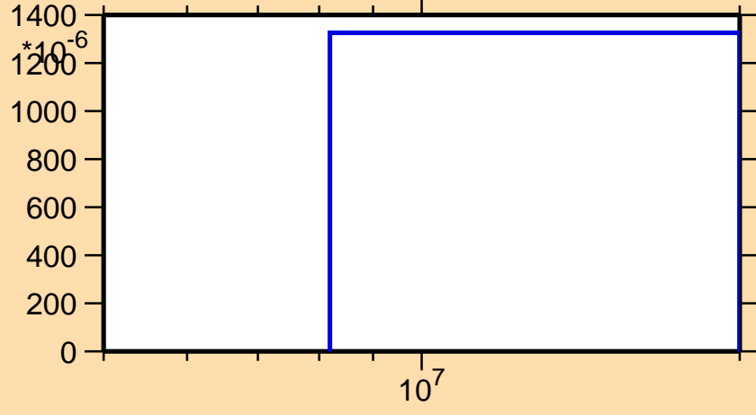
\sigma vs. E for ^{10}\text{C} (mt 45)
