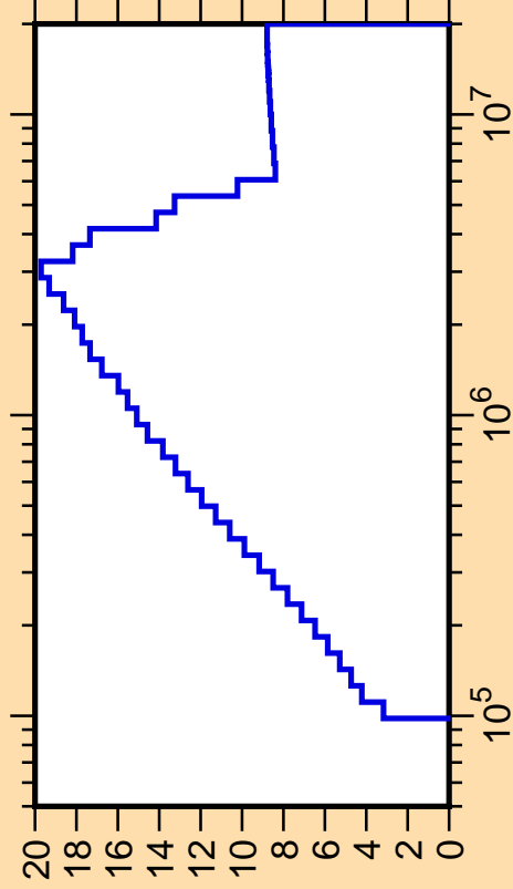
\Delta\mu/\mu vs. E for ^{11}\text{C}(\text{mt251})
