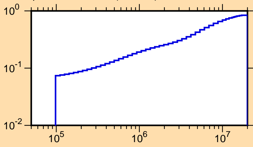
\mu vs. E for ^{11}\text{C}(\text{mt251})
