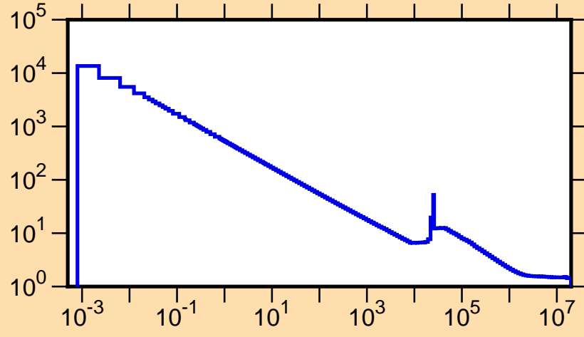
\sigma vs. E for ^{11}\text{C}(n,\text{tot.})
