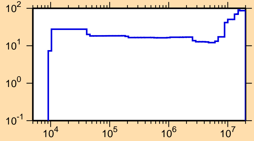
\Delta\sigma/\sigma vs. E for ^{11}\text{C}(n,p)
