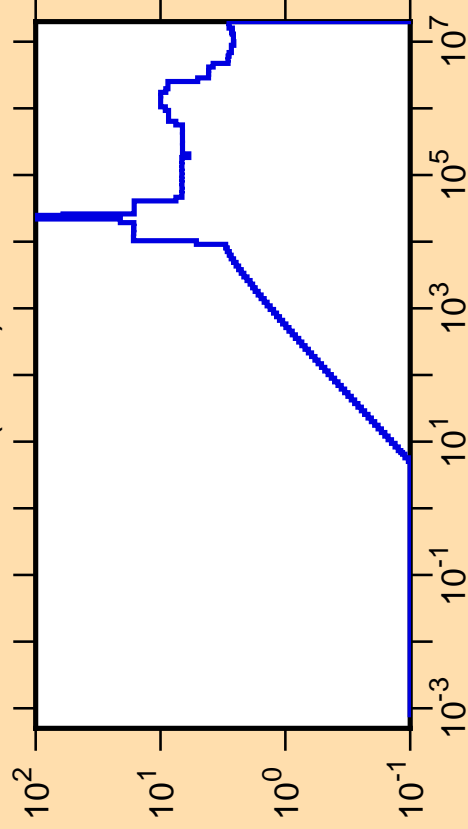
\Delta\sigma/\sigma vs. E for ^{11}\text{C}(n,\text{tot.})
