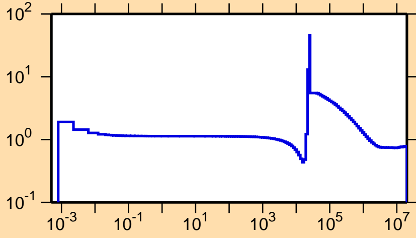
\sigma vs. E for ^{11}\text{C}(n,\text{el.})
