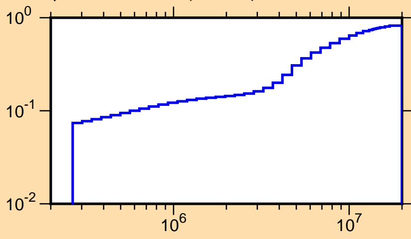
\mu vs. E for ^{13}\text{C}(\text{mt251})
