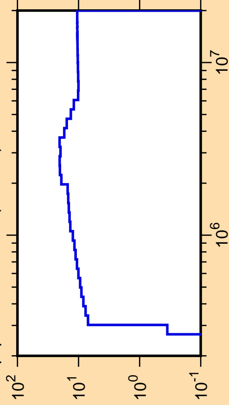
\Delta\mu/\mu vs. E for ^{13}\text{C}(\text{mt251})
