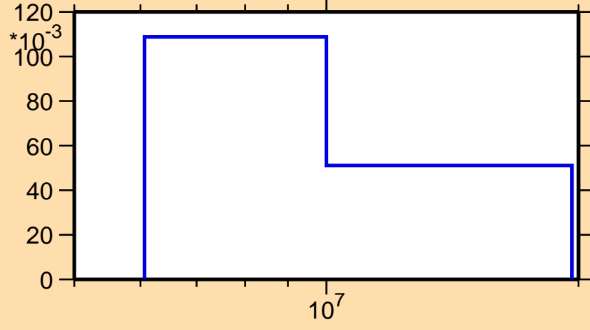
\sigma vs. E for ^{13}\text{C}(n,n_2)
