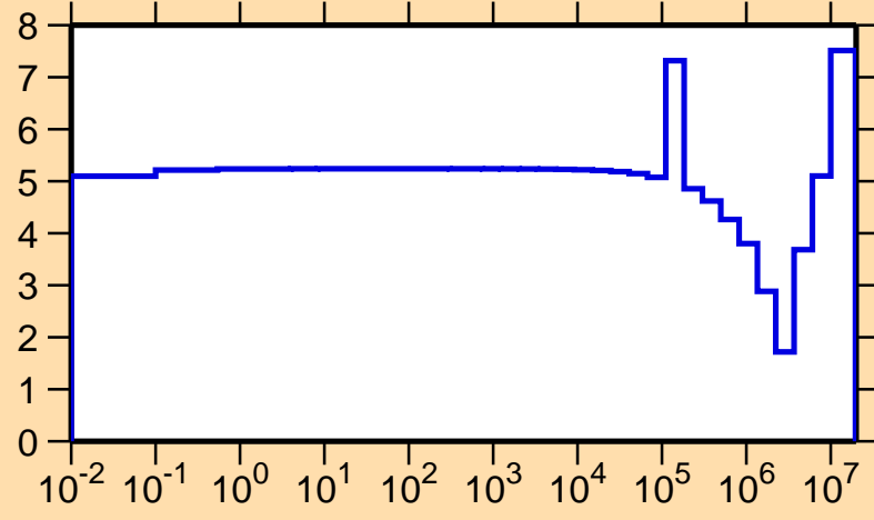
\Delta\sigma/\sigma vs. E for ^{13}\text{C}(n,\text{el.})
