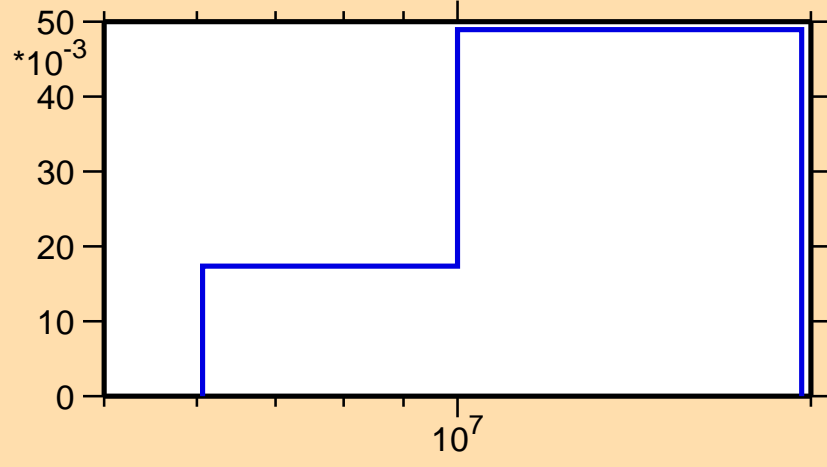
\sigma vs. E for ^{13}\text{C}(n,n_4)
