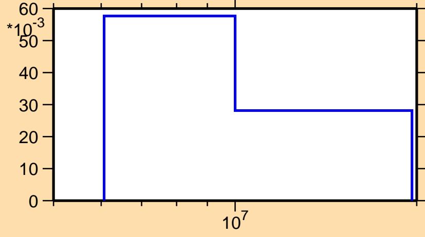
\sigma vs. E for ^{13}\text{C}(n,n_1)
