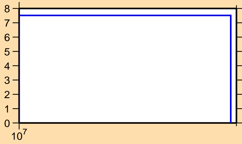
\Delta\sigma/\sigma vs. E for ^{13}\text{C}(n,el.)
